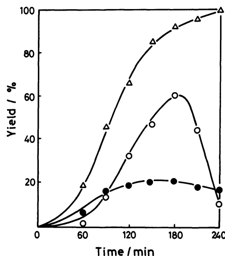
Fig. 2. The time course of p -methoxytoluene oxidation with \text{Co}(\text{OAc})_2\text{-Mn}(\text{OAc})_2 catalyst. \text{Co}(\text{OAc})_2 \cdot 4\text{H}_2\text{O}\text{-Mn}(\text{OAc})_2 \cdot 4\text{H}_2\text{O} (3:2), 0.75 mmol; \text{O}_2 , 3 atm; p -methoxytoluene, 2.0 mmol; AcOH, 10 ml; at 110 °C. ( \Delta ) Conversion, (O) p -anisaldehyde, (●) p -anisyl acetate.
